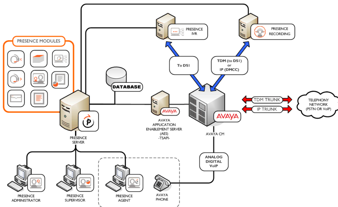
Integrating the Presence Suite with Avaya
